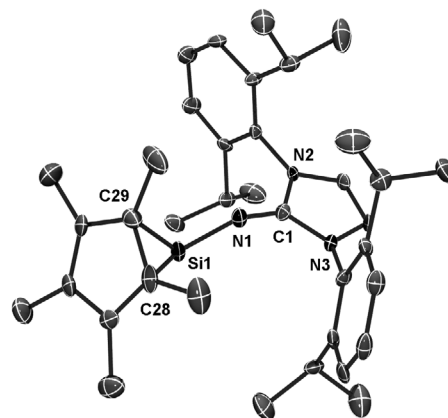
Figure 1. Molecular structure of compound 3 . Thermal ellipsoids are shown at 50 % probability. Hydrogen atoms are omitted for clarity. Selected bond lengths (Å) and angles ( ^\circ ): \text{Si}1-\text{N}1 , 1.691(5); \text{Si}1-\text{C}28 , 2.218(6); \text{Si}1-\text{C}29 , 2.124(6); \text{C}1-\text{N}1 , 1.280(6); \text{C}1-\text{N}2 , 1.377(6); \text{C}1-\text{N}3 , 1.387(6); \text{N}1-\text{Si}1-\text{C}28 , 103.9(2) ; \text{N}1-\text{Si}1-\text{C}29 , 99.5(3) ; \text{Si}1-\text{N}1-\text{C}1 , 136.6(4) .
