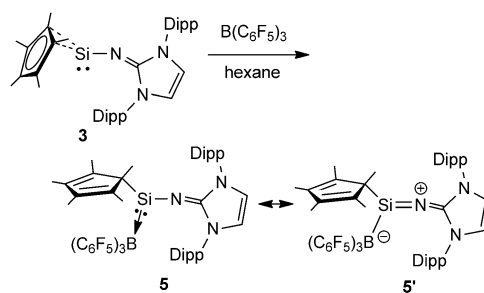
Scheme 4. Synthesis of borane adduct 5 .
